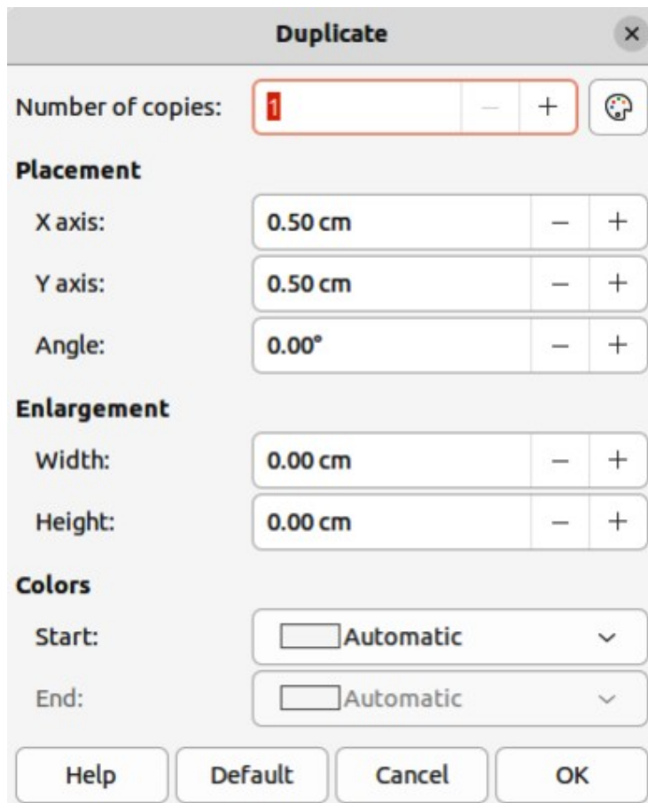
Figure 10: Duplicate dialog
