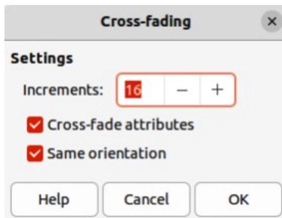
Figure 12: Cross-fading dialog
