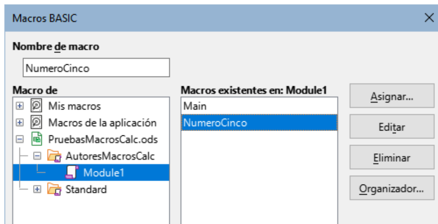
Figura 477: Macros Basic.
