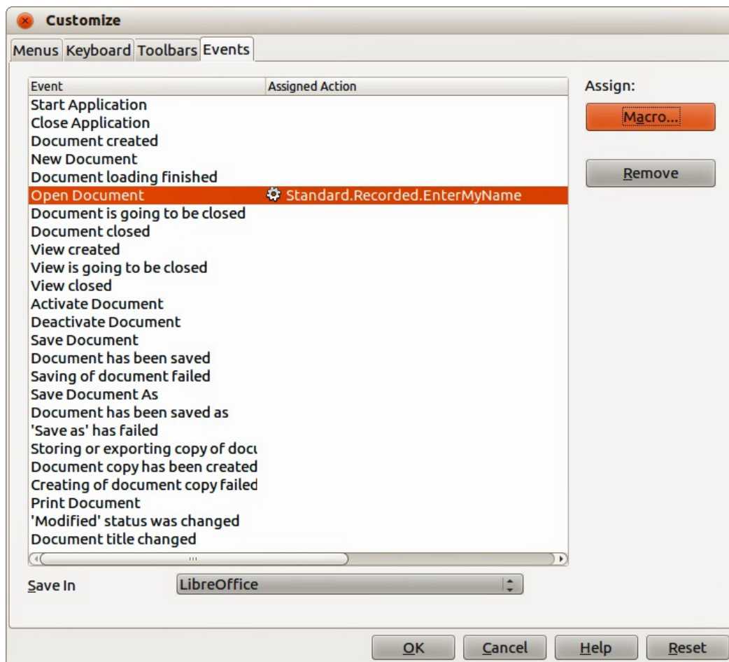
Figure 10: Events page in Customize dialog
