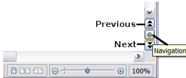
Figure 6: Navigation icons
