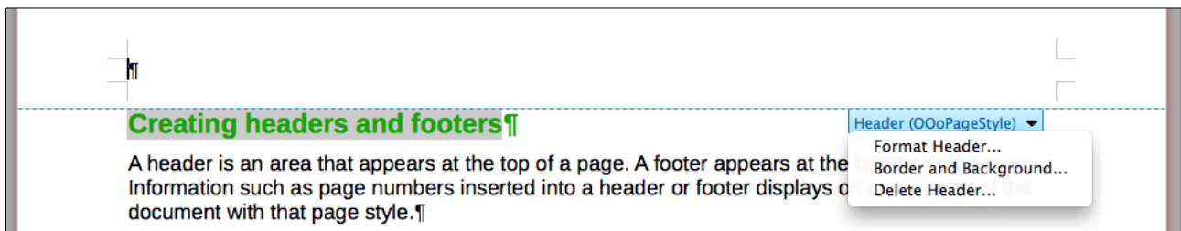
Figure 24: Header menu
