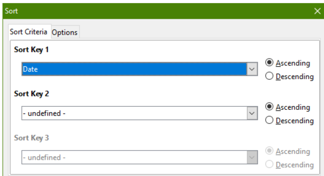
Figure 37: Sort dialog – Sort Criteria tab
