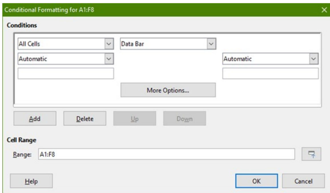
Figure 27: Conditional Formatting dialog – Data Bar
