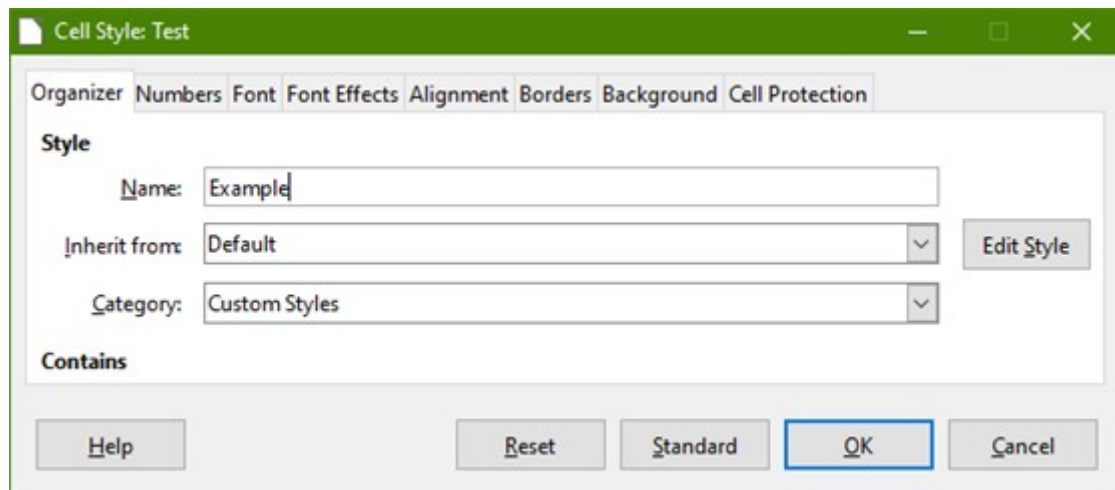
Figure 28: Cell Style dialog
