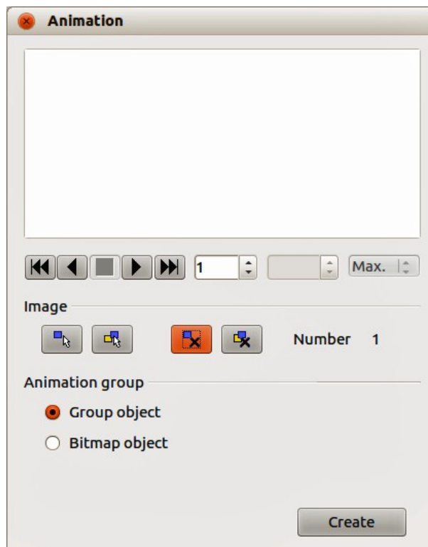
Figure 24: Animation dialog
