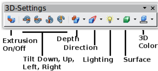
Figure 16: 3D-Settings toolbar
