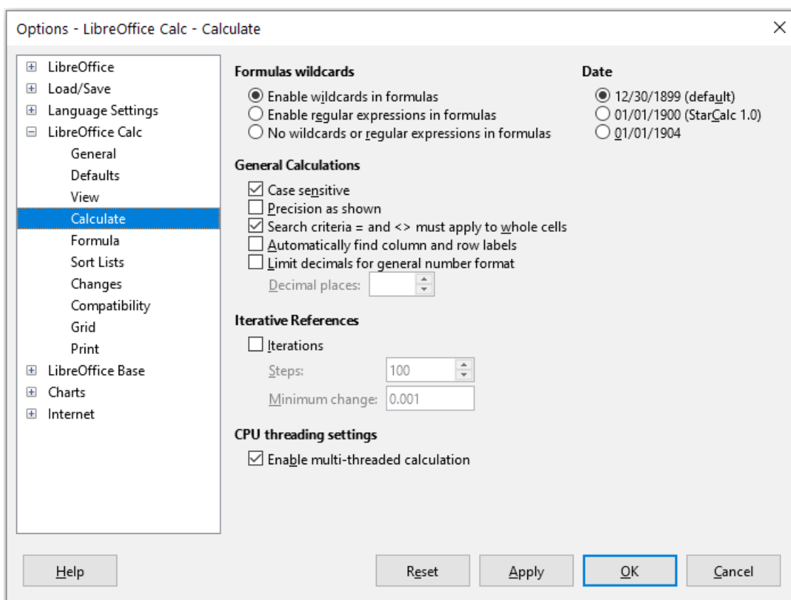
Figure 28: Tools > Option > LibreOffice Calc > Calculate dialog
