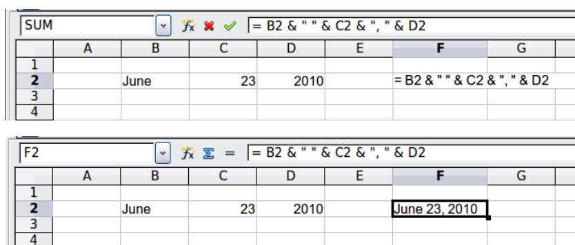
Figure 3: Text concatenation
