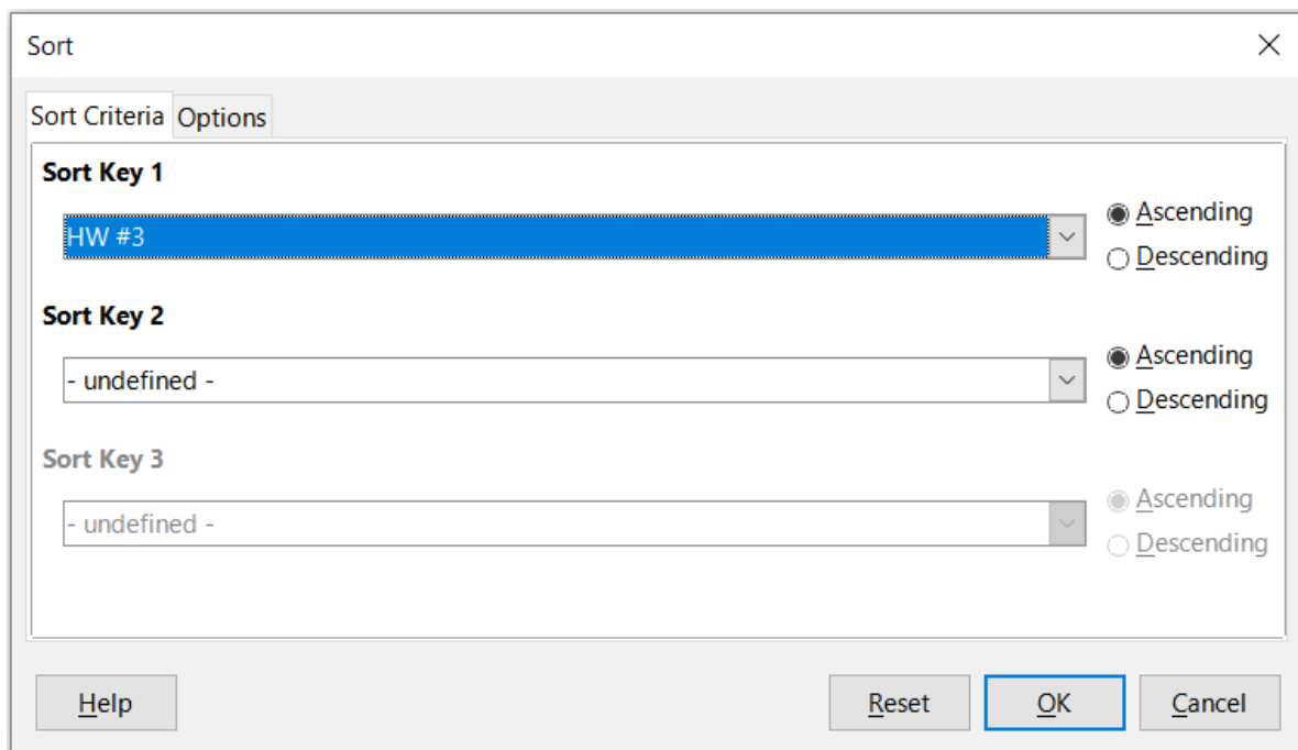
Figure 8: Sort dialog
