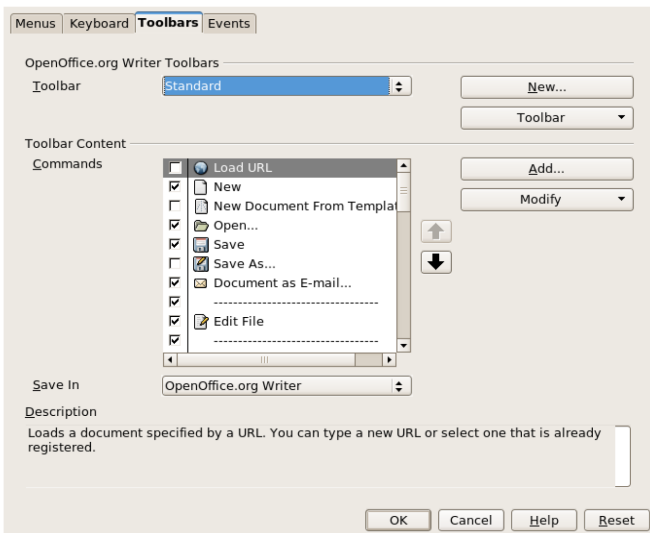
Figure 11: OpenOffice.orgLibreOffice Customize dialog
