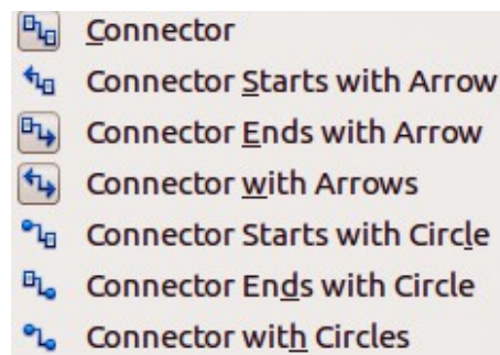
Figure 2: Standard connectors
