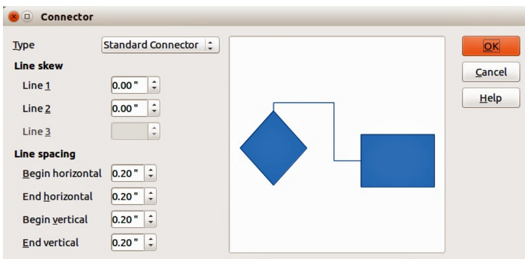
Figure 7: Connector dialog
