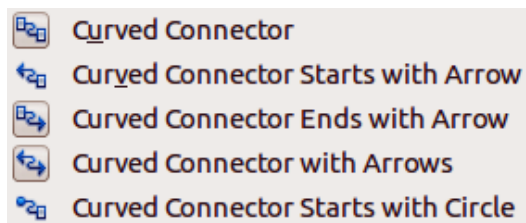
Figure 5: Curved connectors
