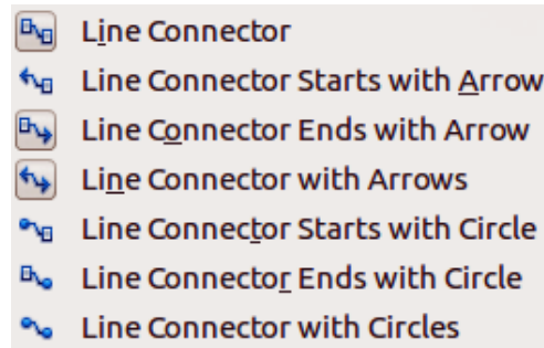
Figure 3: Line connectors
