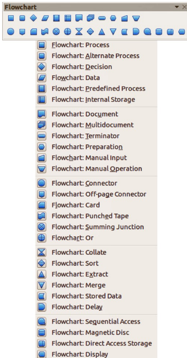
Figure 10: Flowchart toolbar
