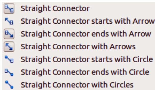
Figure 4: Straight connectors
