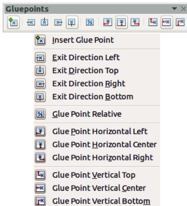
Figure 8: Gluepoints toolbar
