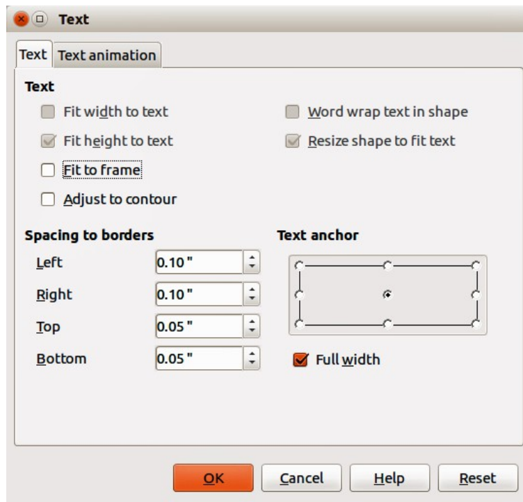
Figure 9: Text dialog
