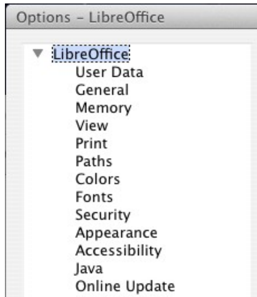
Figure 1: LibreOffice options
