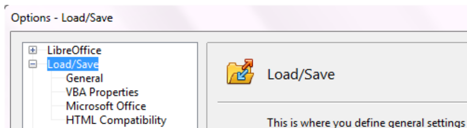
Figure 18: Load/Save options
