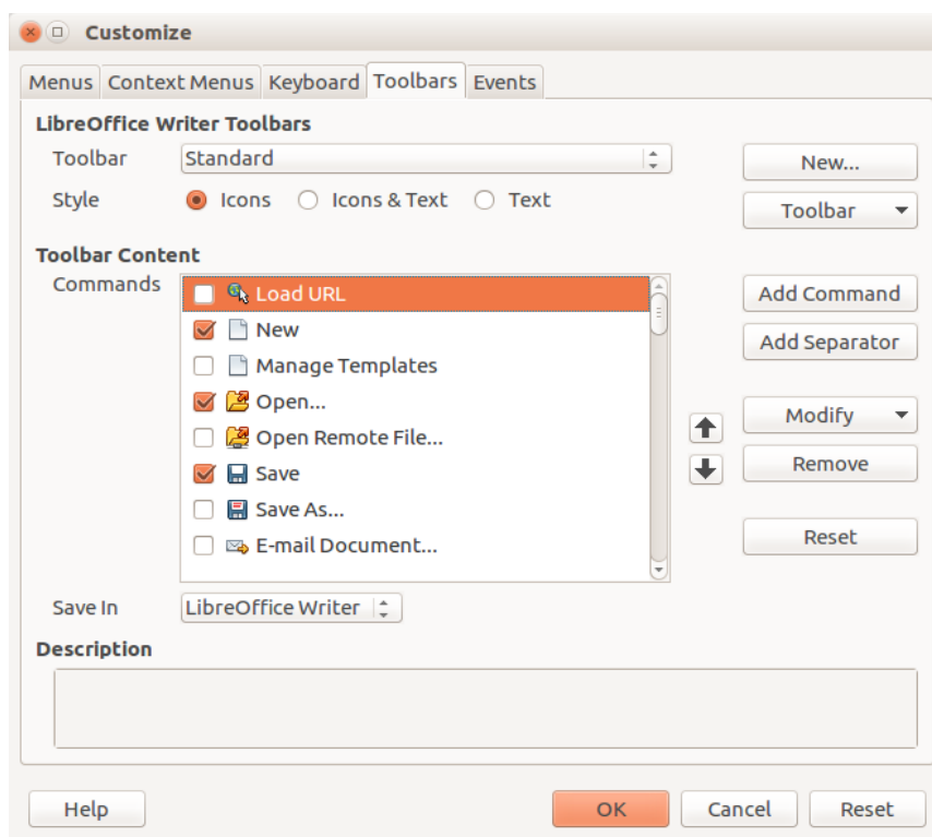
Figure 4: The Toolbars page of the Customize dialog
