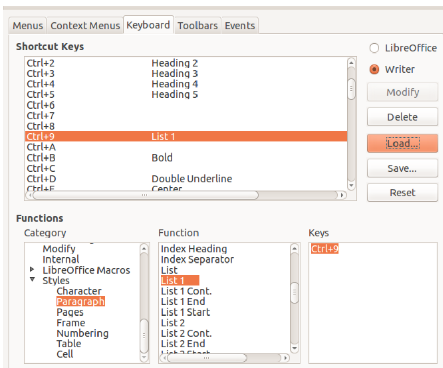
Figure 9: Defining keyboard shortcuts for applying styles
