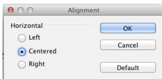
Figure 19: Alignment dialog
