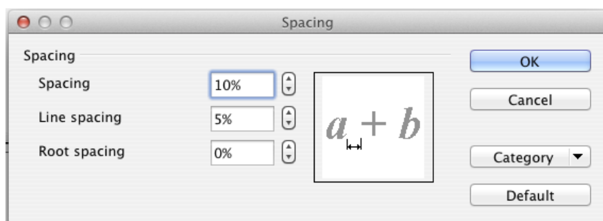
Figure 18: Spacing dialog
