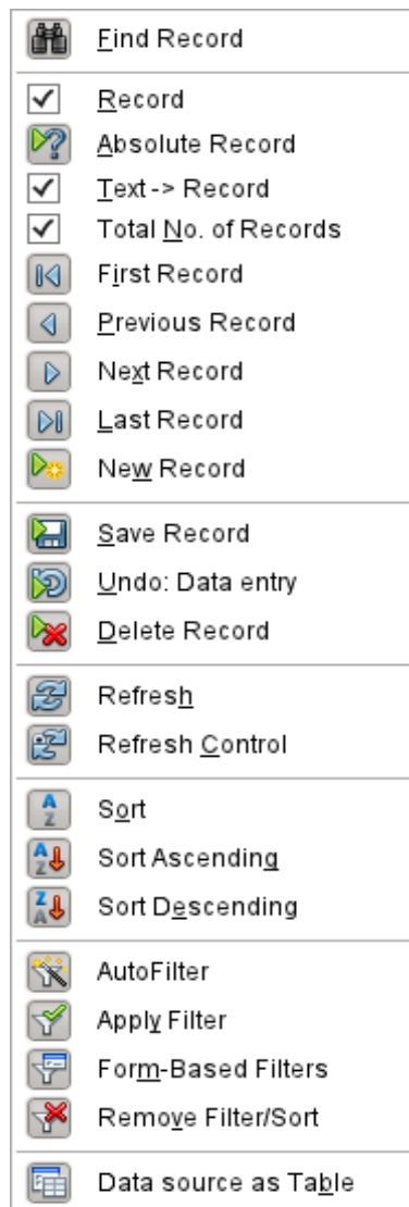
Figure 30: Navigation buttons
