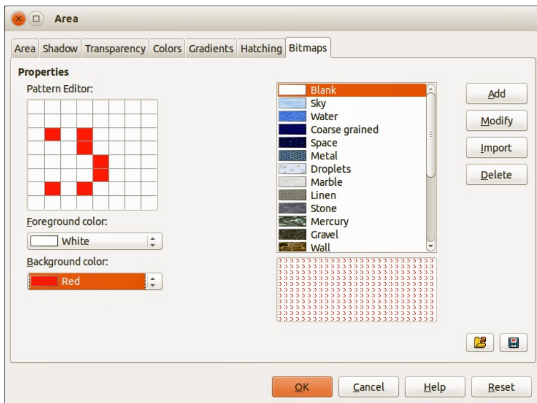
Figure 23: Area dialog – Bitmaps page
