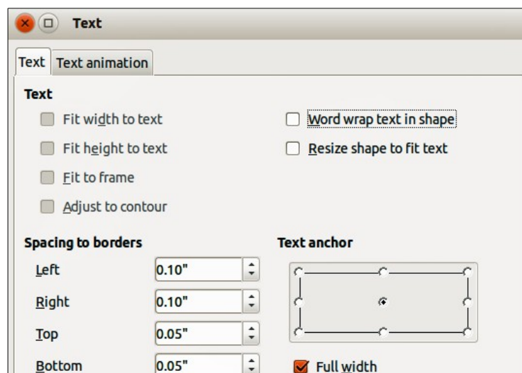
Figure 26: Text dialog
