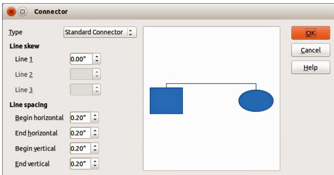
Figure 28: Connector dialog
