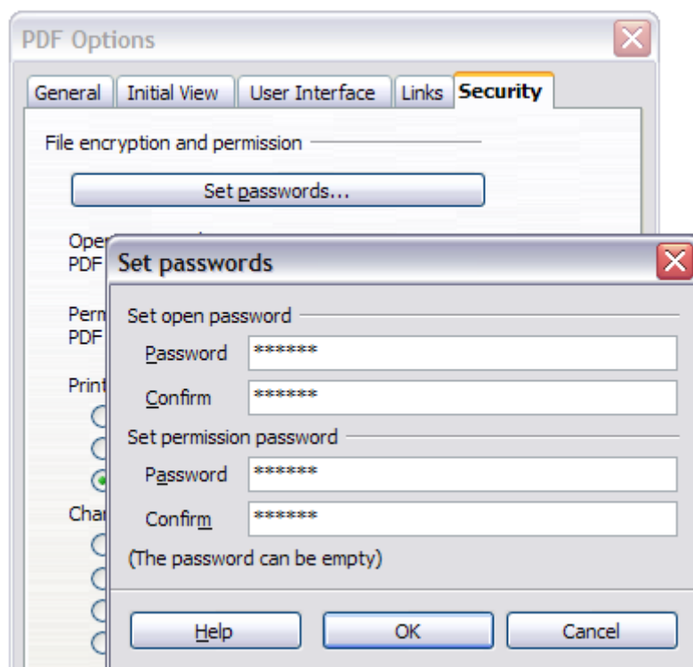
Figure 154: Setting a password to encrypt a PDF
