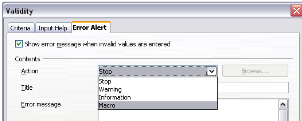
Figure 48: Defining an error message for a cell with invalid data
