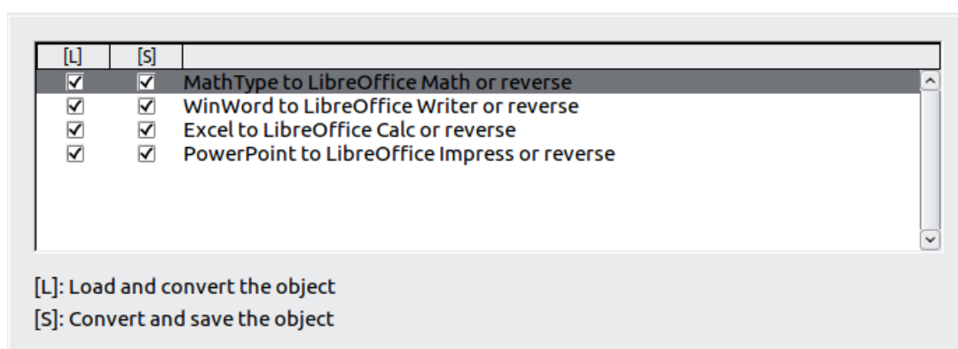
Figure 331: Choosing Load/Save Microsoft Office options
