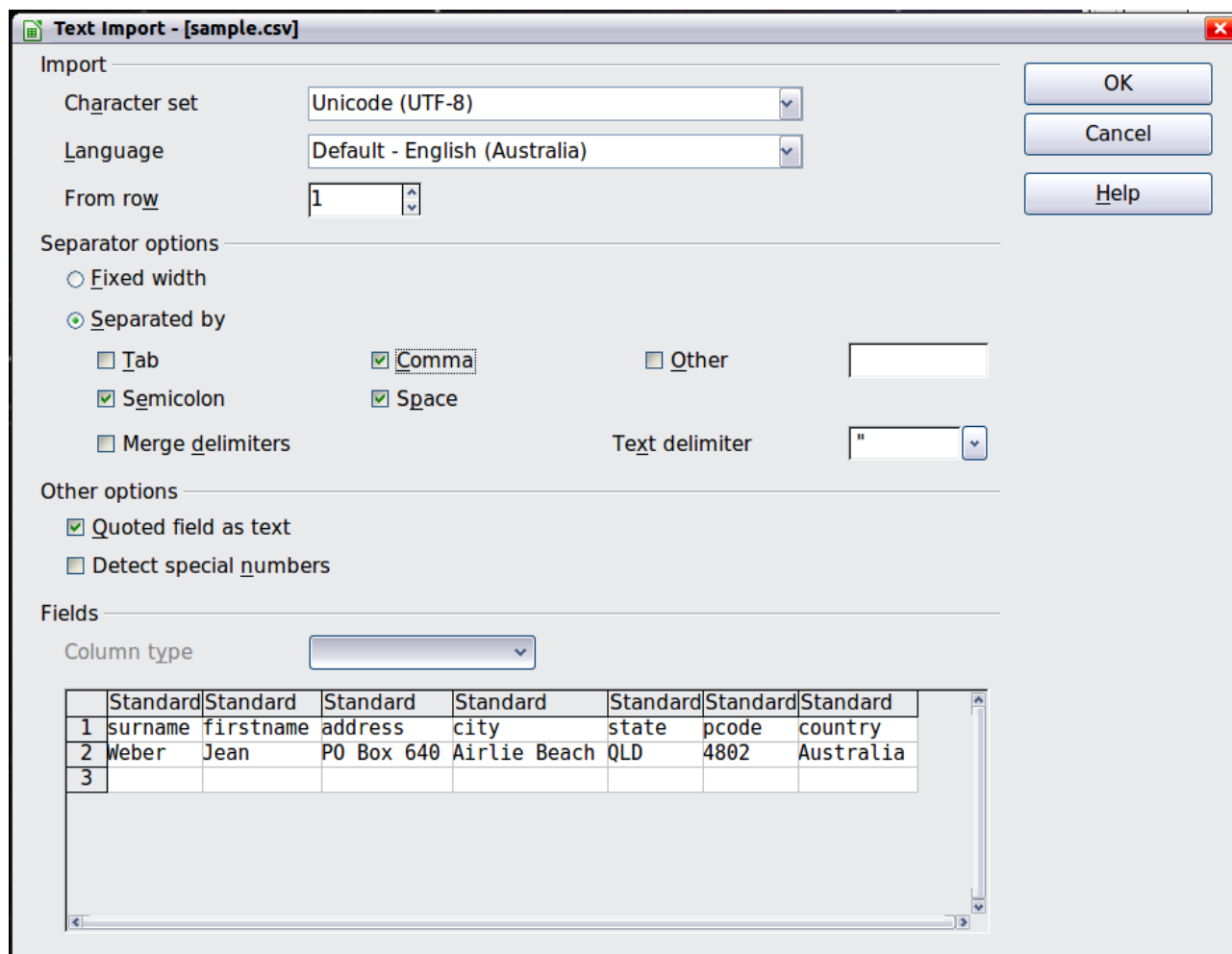
Figure 17: Text Import dialog, with Comma (,) selected as the separator and double quotation mark (") as the text delimiter.
