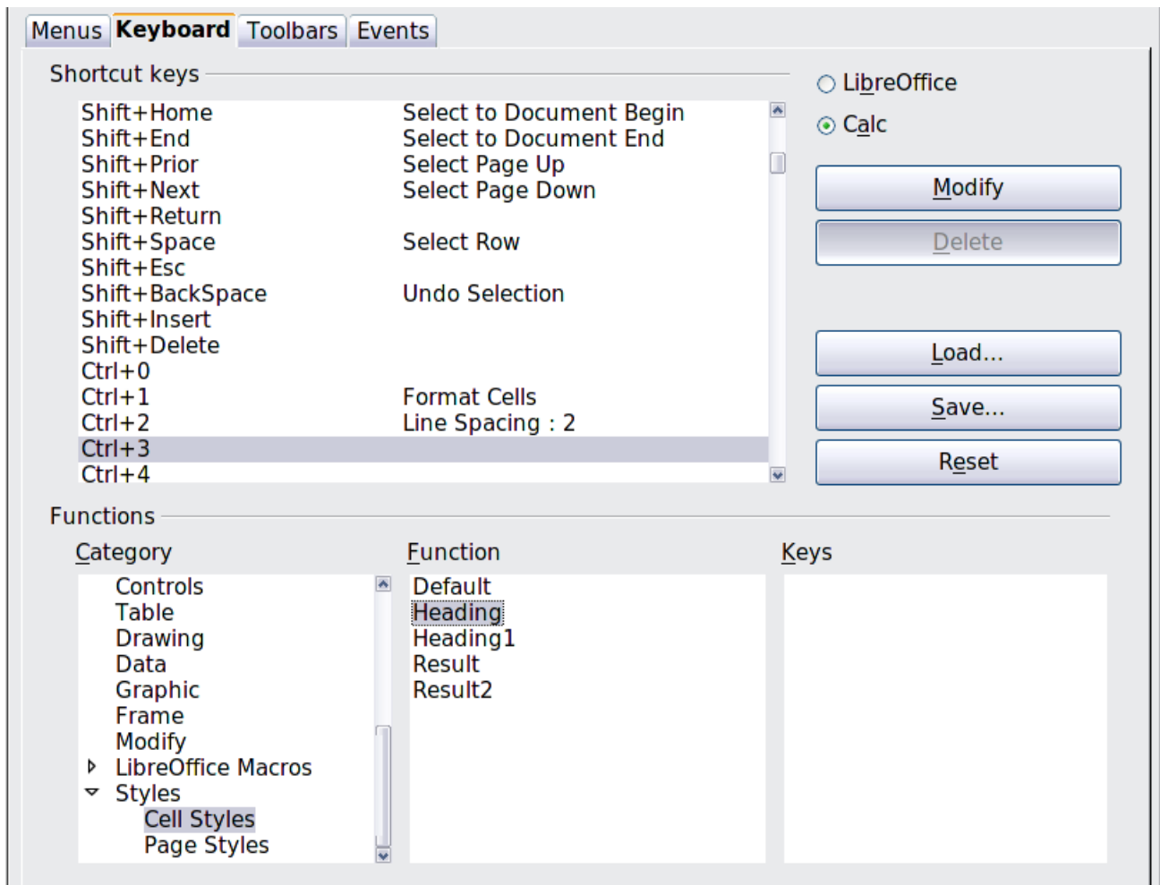
Figure 348: Assigning a cell style to a key combination
