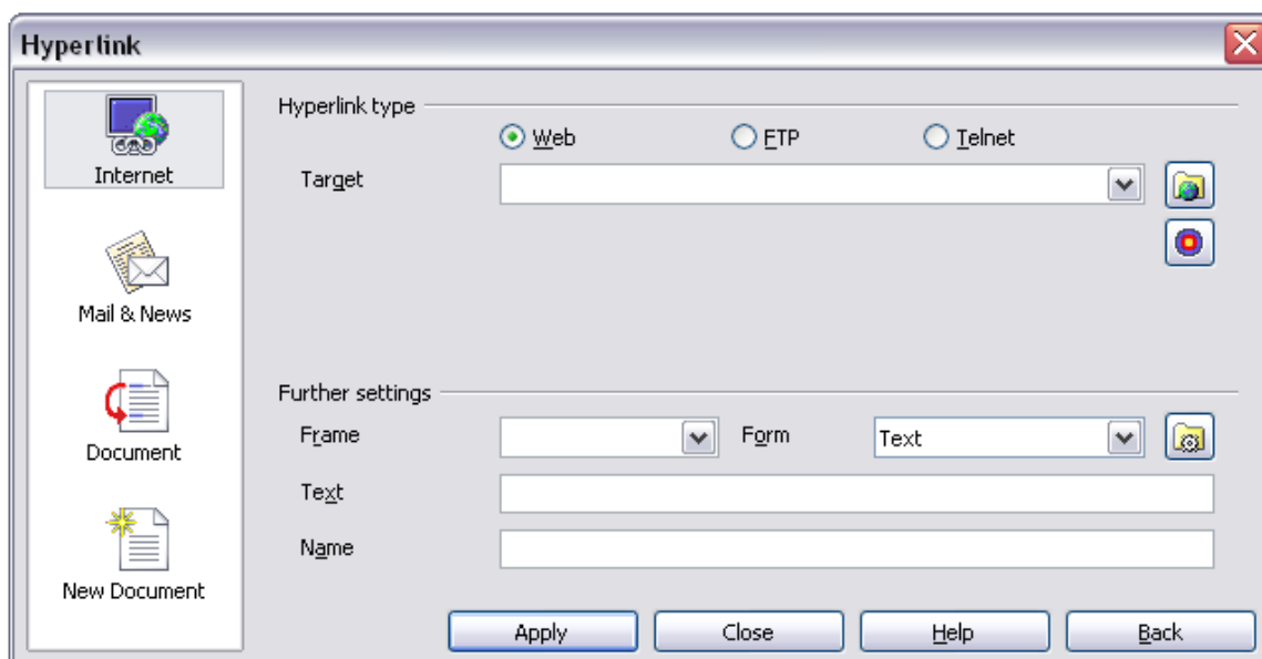
Figure 261. Hyperlink dialog showing details for Internet links
