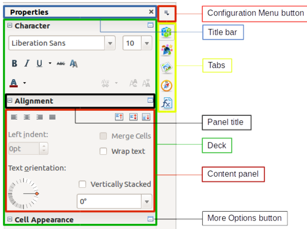
Figure 5: Calc Sidebar with Properties open
