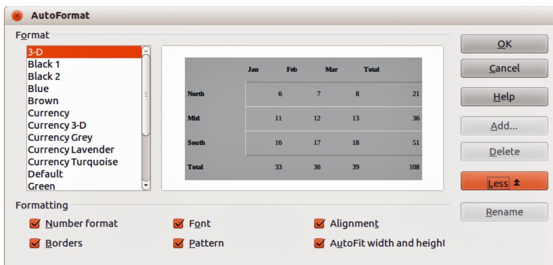
Figure 35: AutoFormat dialog
