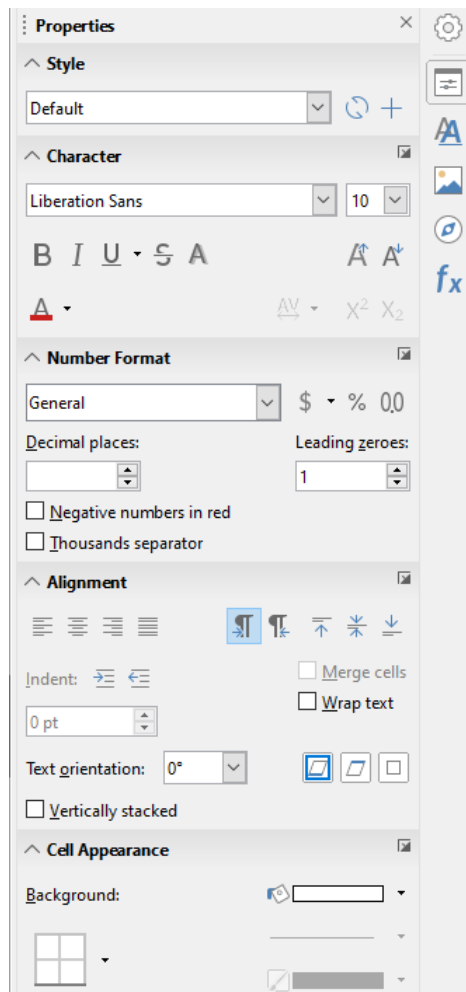
Figure 6: Sidebar
