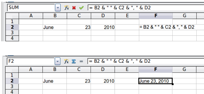
Figure 206: Text concatenation
