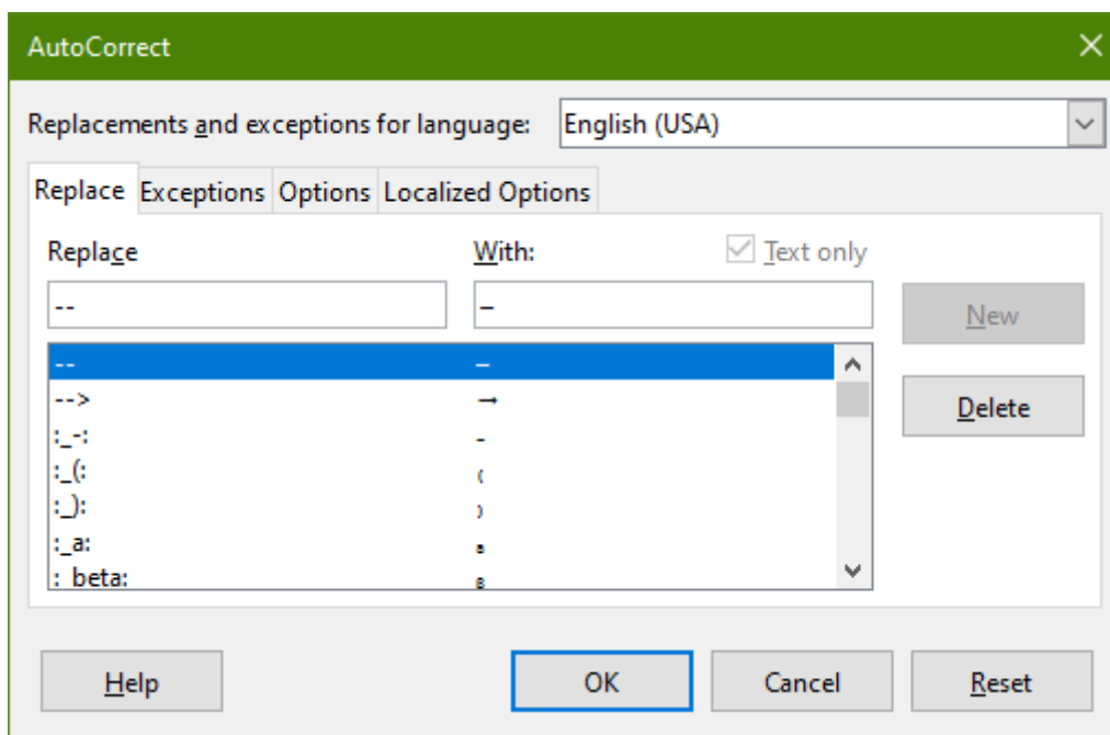
Figure 26: AutoCorrect dialog
