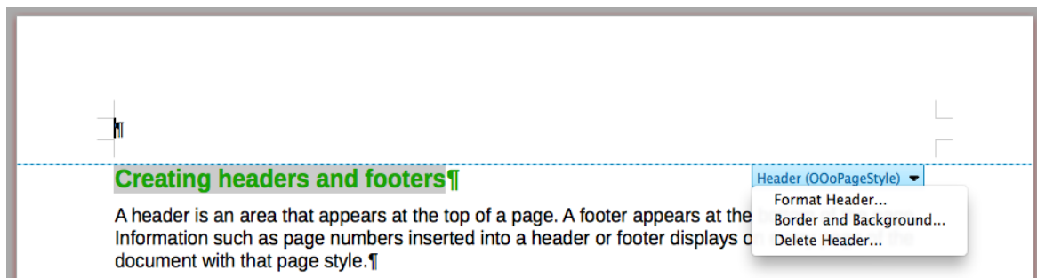
Figure 21: Header menu
