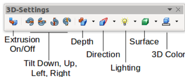
Figure 16: 3D-Settings toolbars
