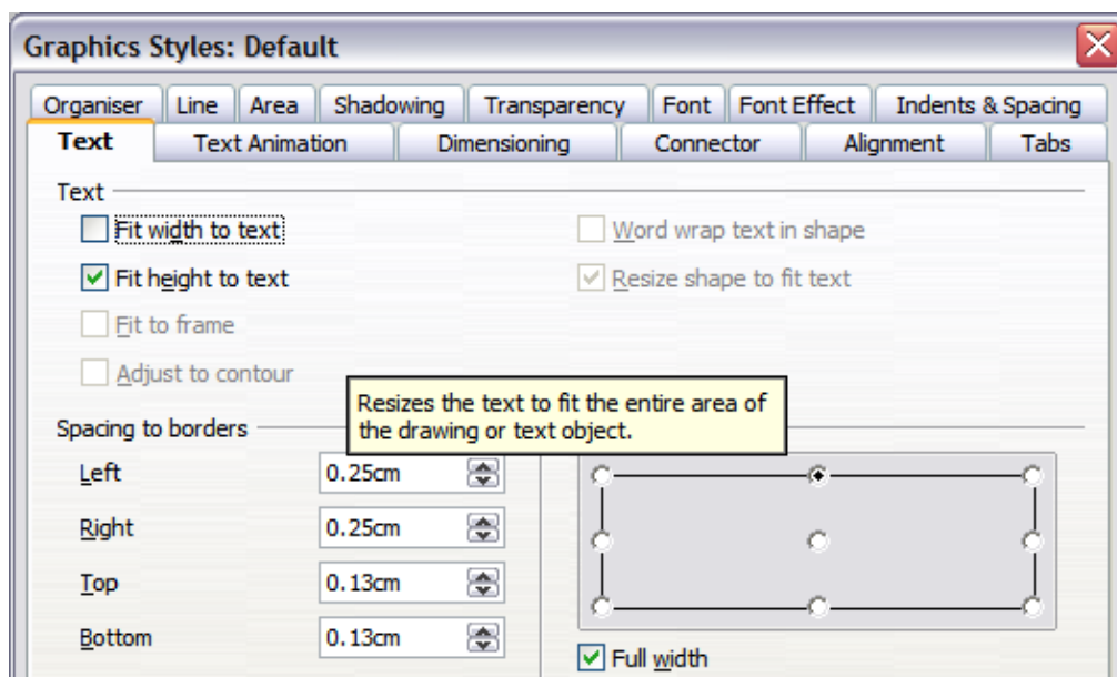
Figure 233: Text tab of Graphic Styles dialog
