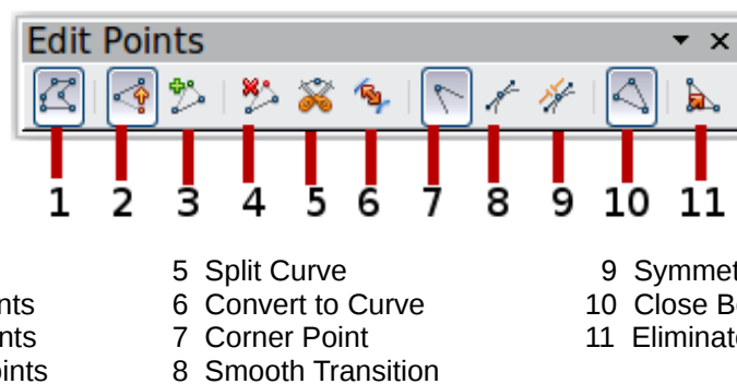
Figure 53: Edit Points toolbar
