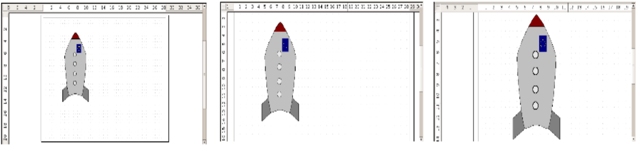
Figure 4: Zoom values – Fit width and height, Fit width, and Optimal
