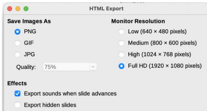
Figure 12: HTML Export dialog – image format, monitor resolution, and effects page
