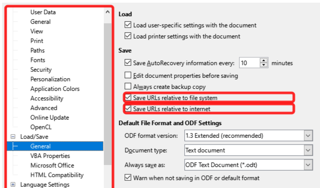
Figure 1: Options for storing hyperlinks
