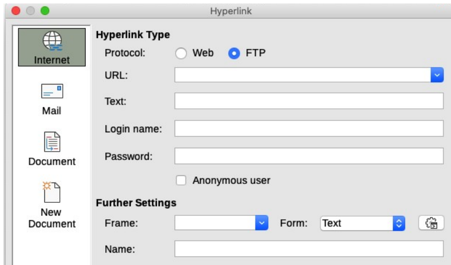
Figure 5: Hyperlink dialog showing details for an Internet FTP link
