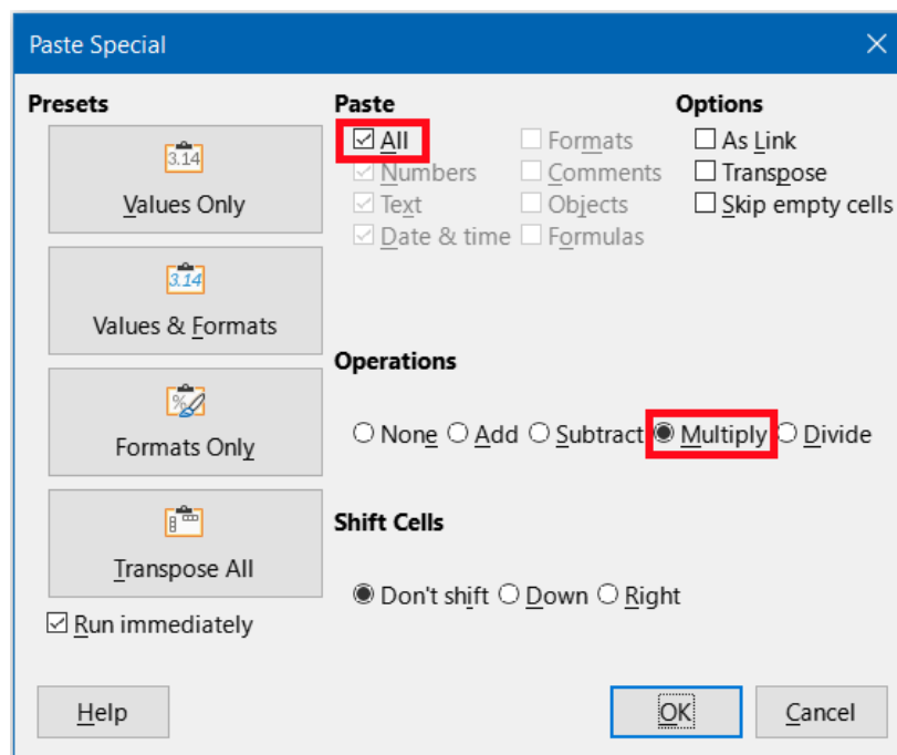
Figure 3: Paste Special dialog
