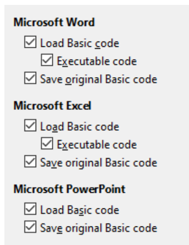
Figure 28: Choosing Load/Save VBA Properties
