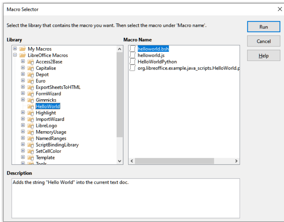
Figure 21: Macro Selector dialog
