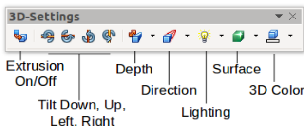
Figure 15: 3D-Settings toolbars
