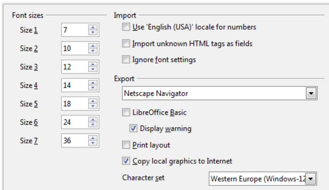
Figure 19: Choosing HTML compatibility options
