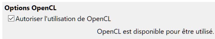
Figure 19 : Options OpenCL
