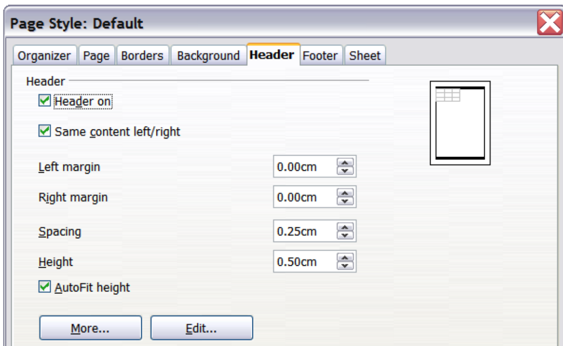
Figure 12: Header dialog
