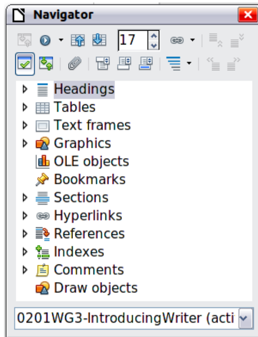
Figure 19. The Navigator
