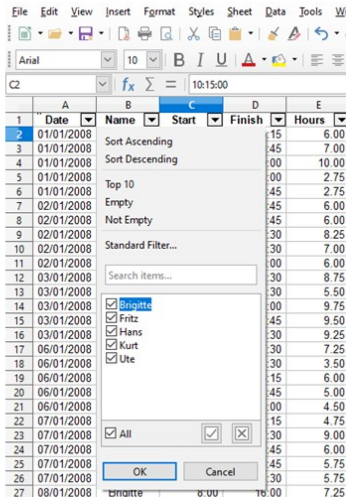
Figure 58: AutoFilter example
