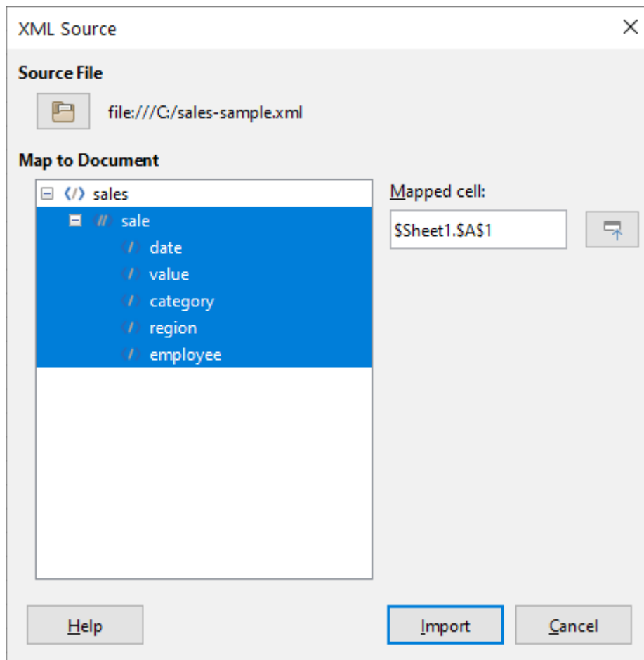
Figure 396: XML Source dialog (populated)
