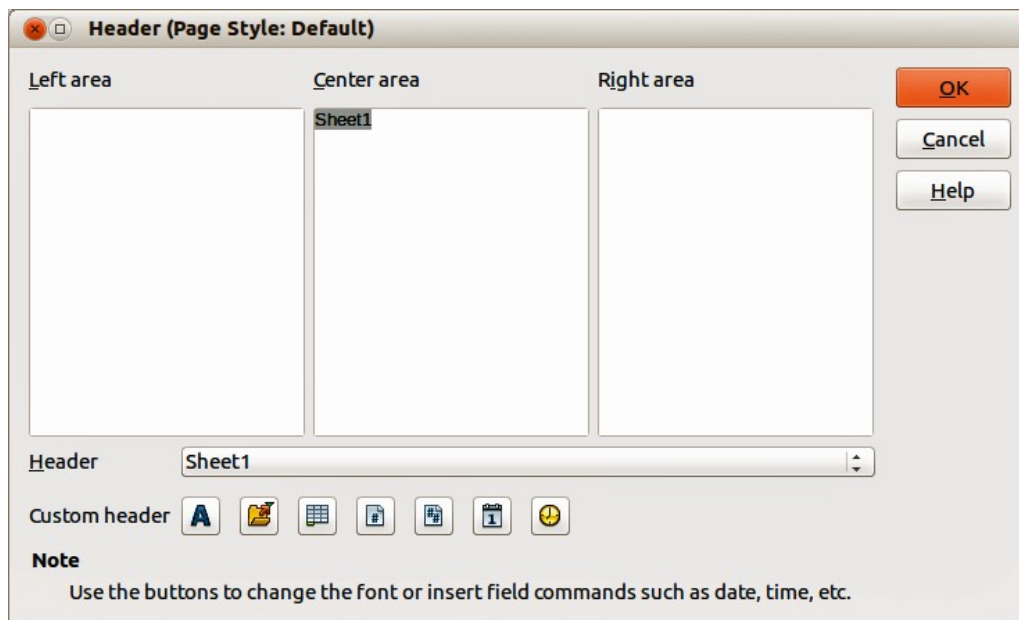
Figure 196: Header dialog
