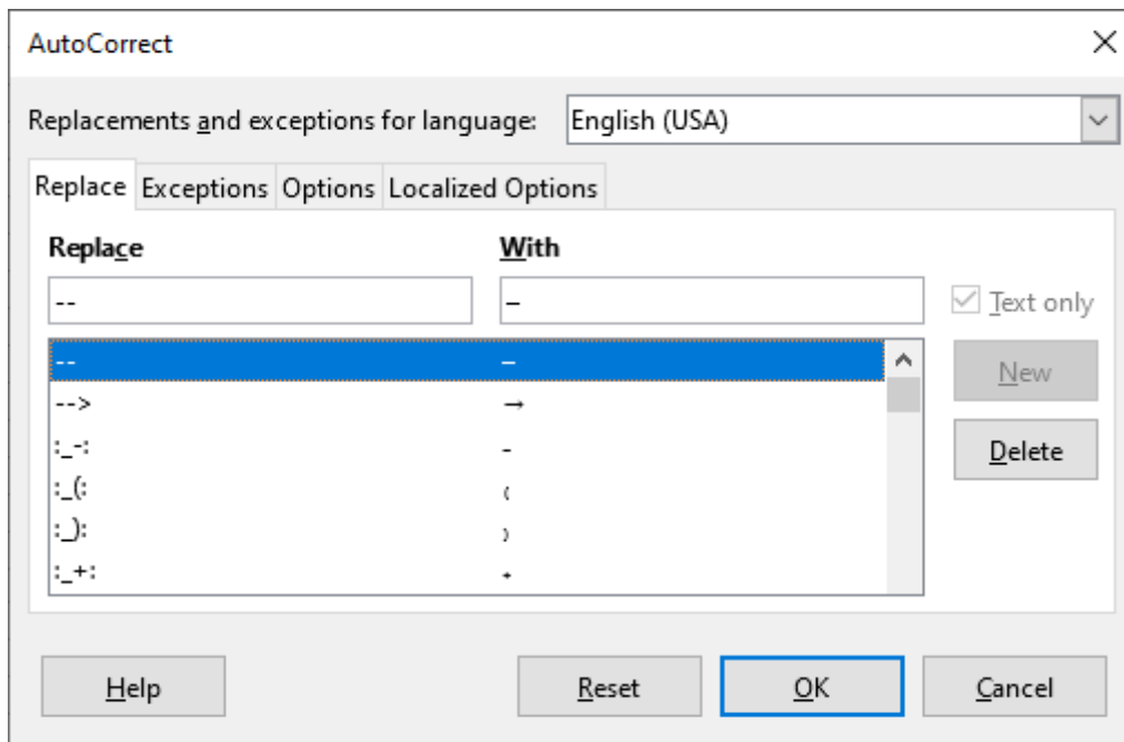
Figure 27: AutoCorrect dialog
