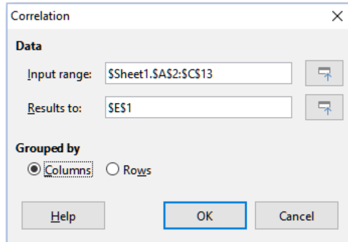
Figure 326: Correlation dialog
