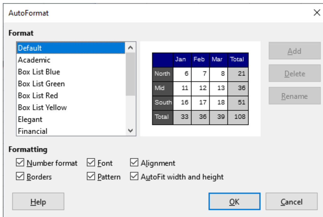
Figure 45: AutoFormat dialog
