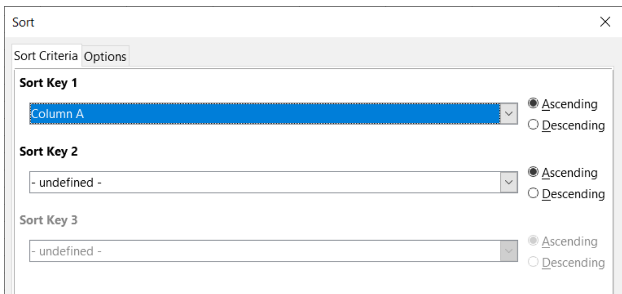
Figure 447: Sort dialog
