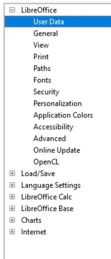
Figure 459: LibreOffice options
