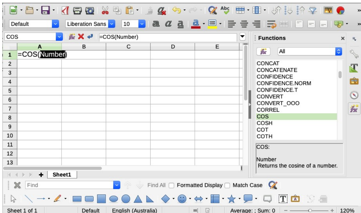
Figure 221: Functions List deck in Sidebar
