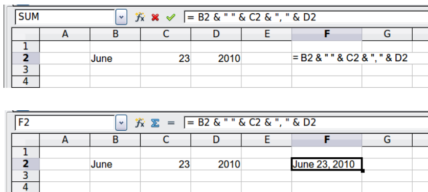
Figure 208: Text concatenation
