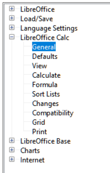
Figure 467: Calc options
