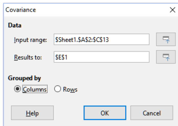
Figure 328: Covariance dialog
