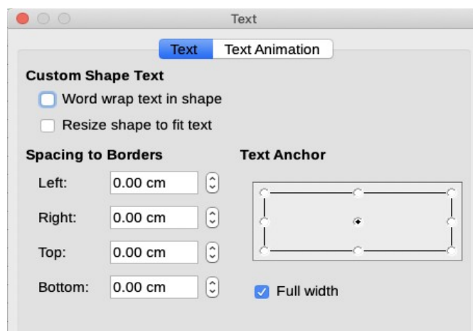
Figure 174: Text dialog
