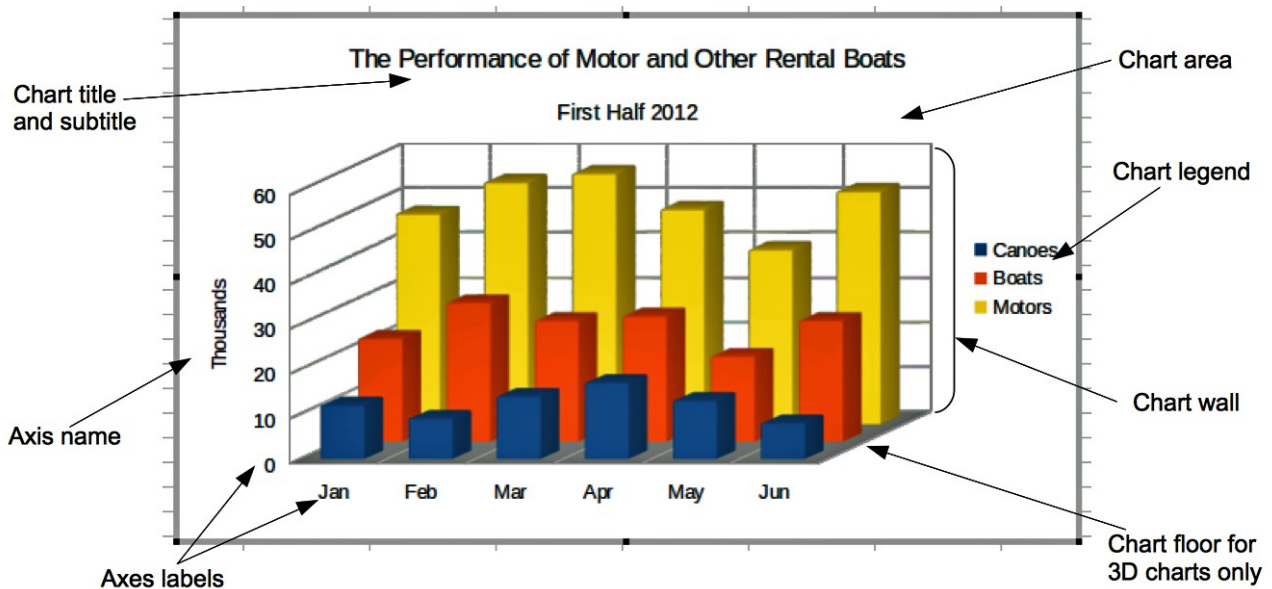
Figure 71: Chart elements
