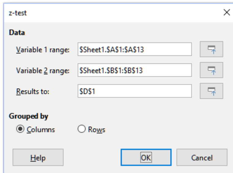
Figure 343: z-test dialog
