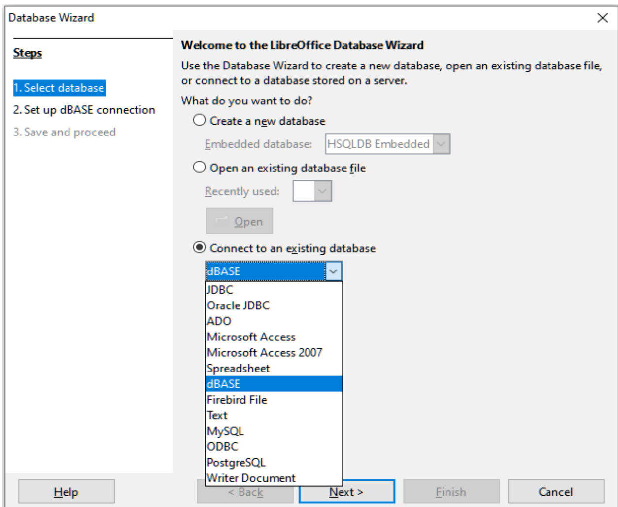
Figure 384: Database Wizard
