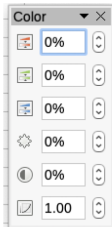
Figure 172: Color toolbar
