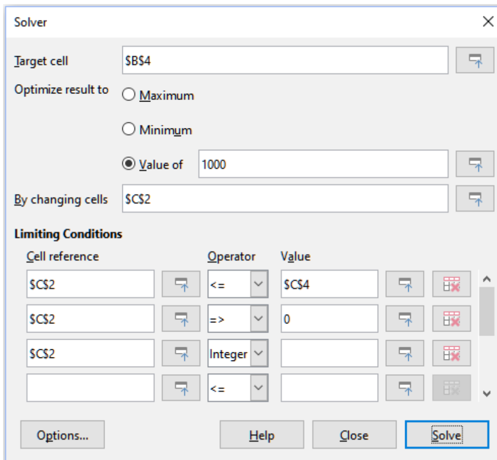
Figure 314: Solver dialog
