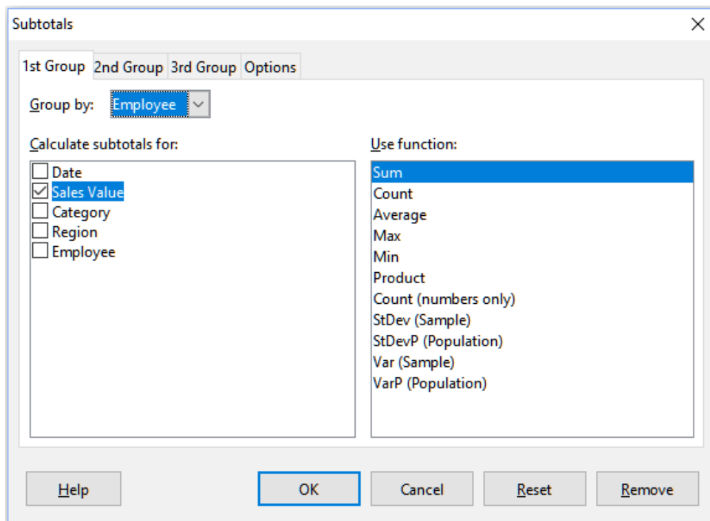
Figure 295: Subtotals dialog
