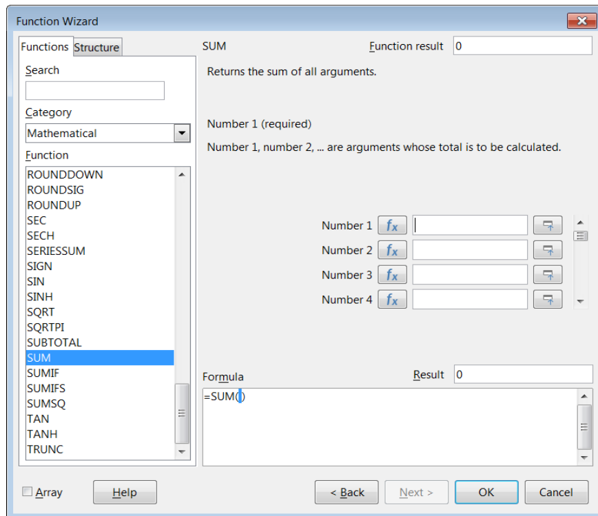
Figure 222: Functions tab of Function Wizard
