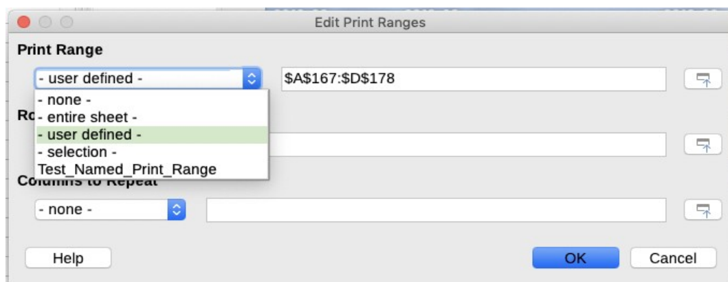
Figure 191: Choosing a named range for printing
