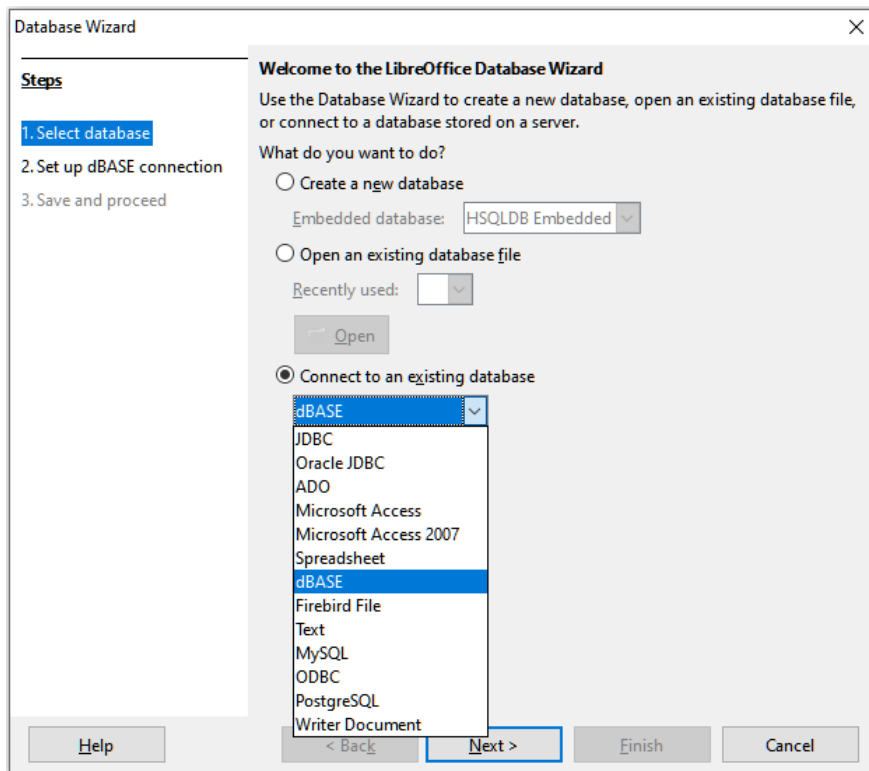
Figure 38: Database Wizard
