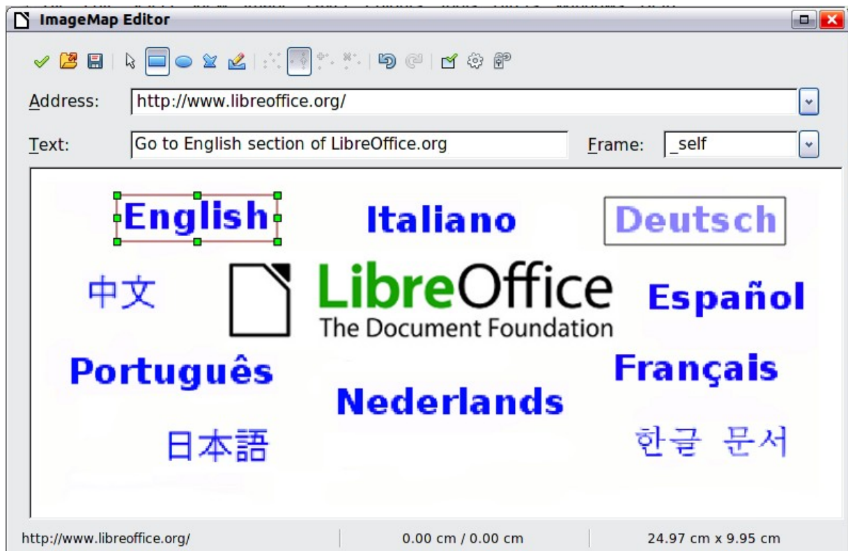
Figure 12: The dialog box to create or edit an image map
