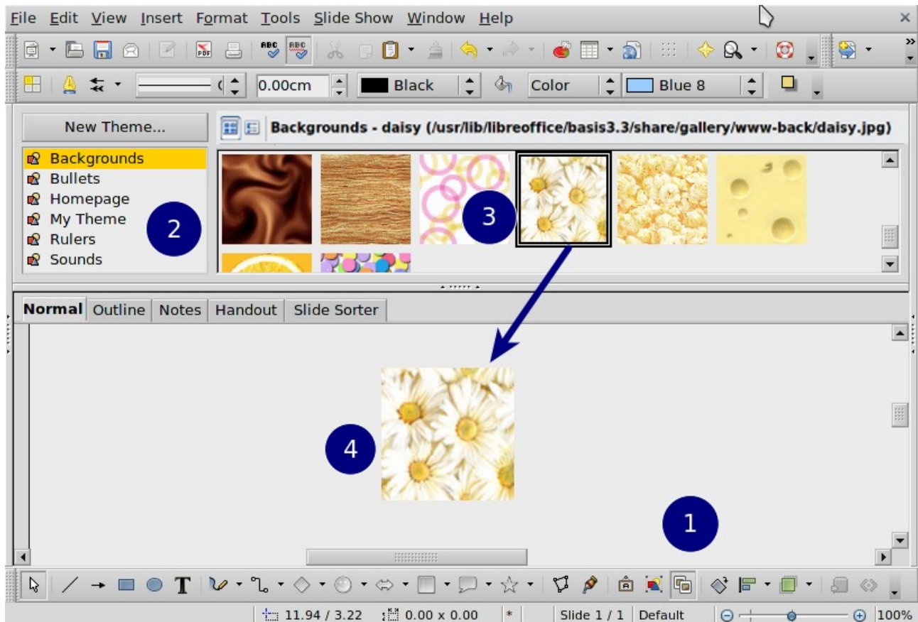
Figure 3. Inserting an image from the Gallery
