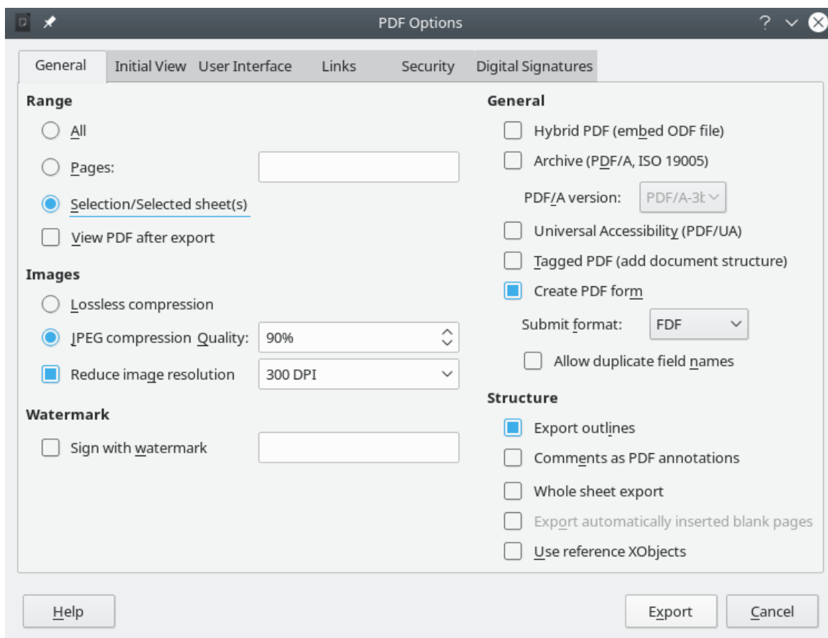
Figure 15: PDF Options dialog – General tab
