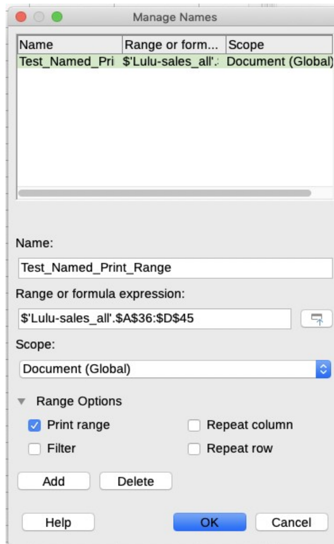
Figure 10: Manage Names dialog
