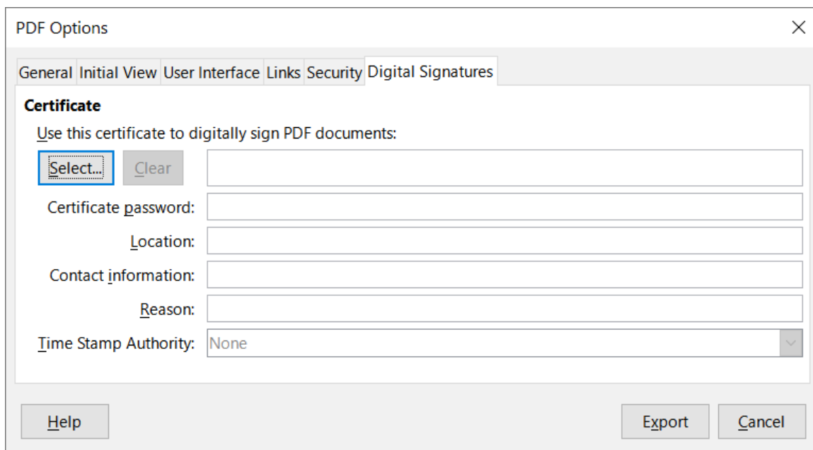
Figure 21: PDF Options dialog – Digital Signatures tab
