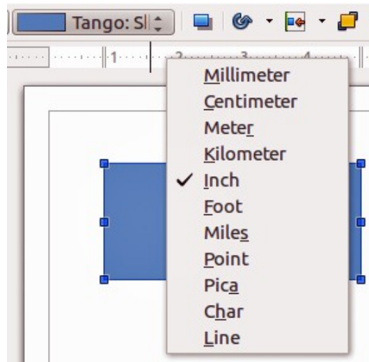
Figure 3: Ruler units
