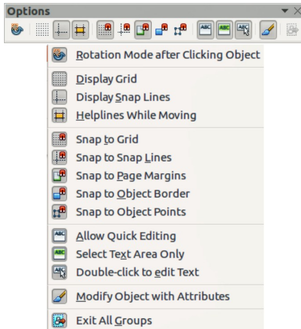
Figure 10: Options toolbar
