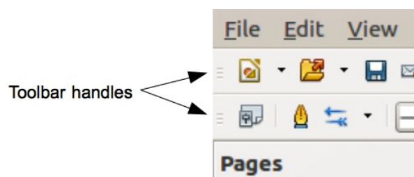
Figure 12: Toolbar handles
